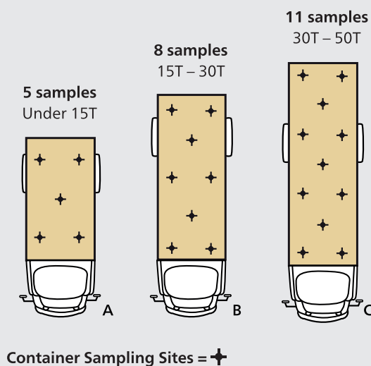
Figure 1: Number of samples to take from containers of various sizes
